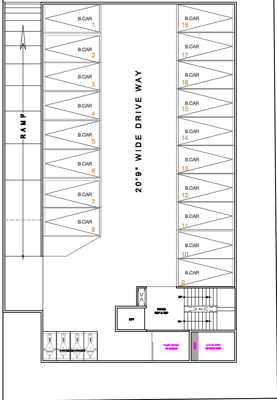
BASEMENT PLAN
